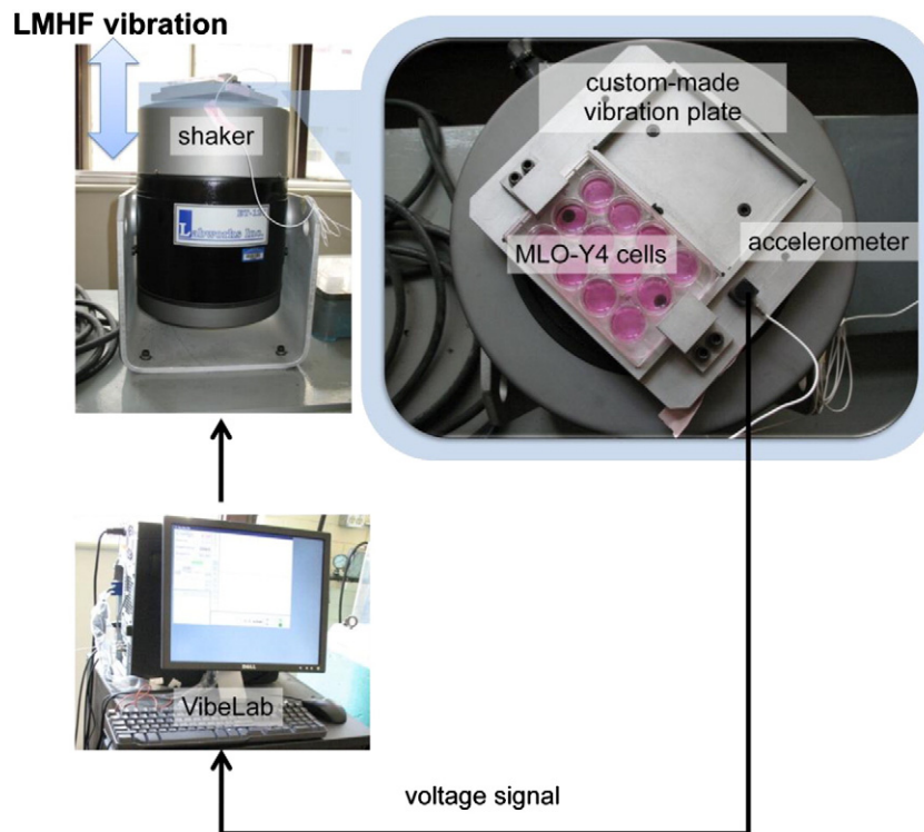
Fig. 1. Experimental set-up. A rigid vibration plate was custom-made to fit two standard multi-well tissue culture plates. LMHF vibration was delivered through a vibration shaker controlled by a feedback loop consisting of an accelerometer attached to the vibration plate and a computer equipped with a VibeLab user interface.
